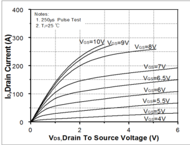
Fig. 1. On-state characteristics
