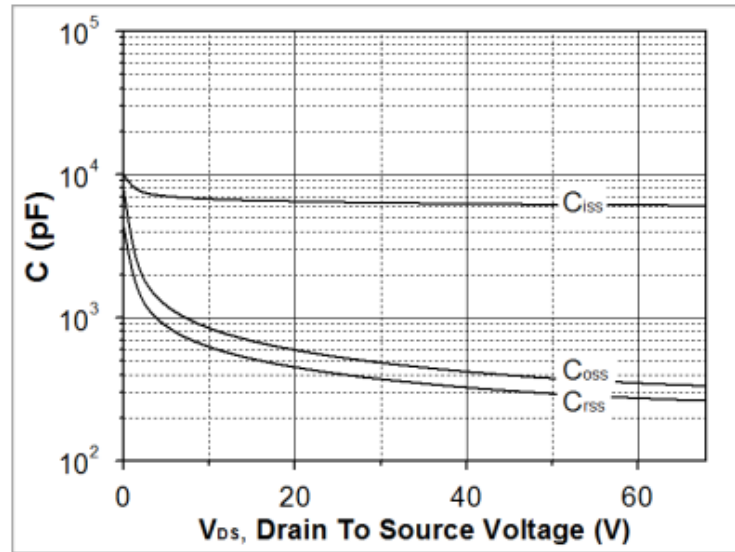
Fig. 8. Capacitance Characteristics
