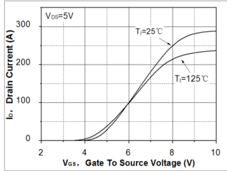
Fig. 2. Transfer Characteristics
